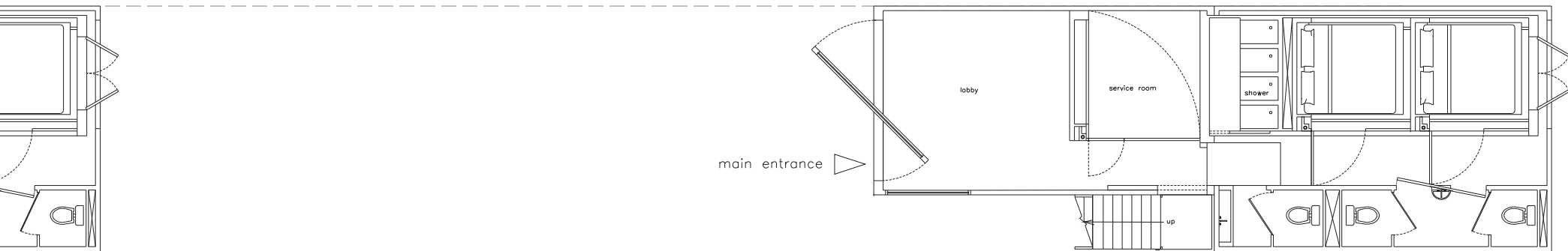
HOTEL 1F PLAN SCALE : 1/100
