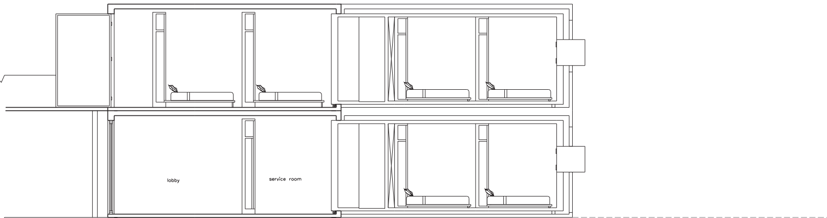
HOTEL SECTION EE' SCALE : 1/100
