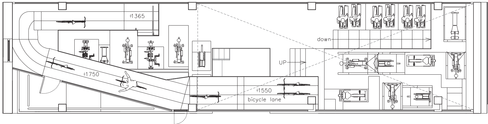
GYM 6F PLAN SCALE : 1/100
