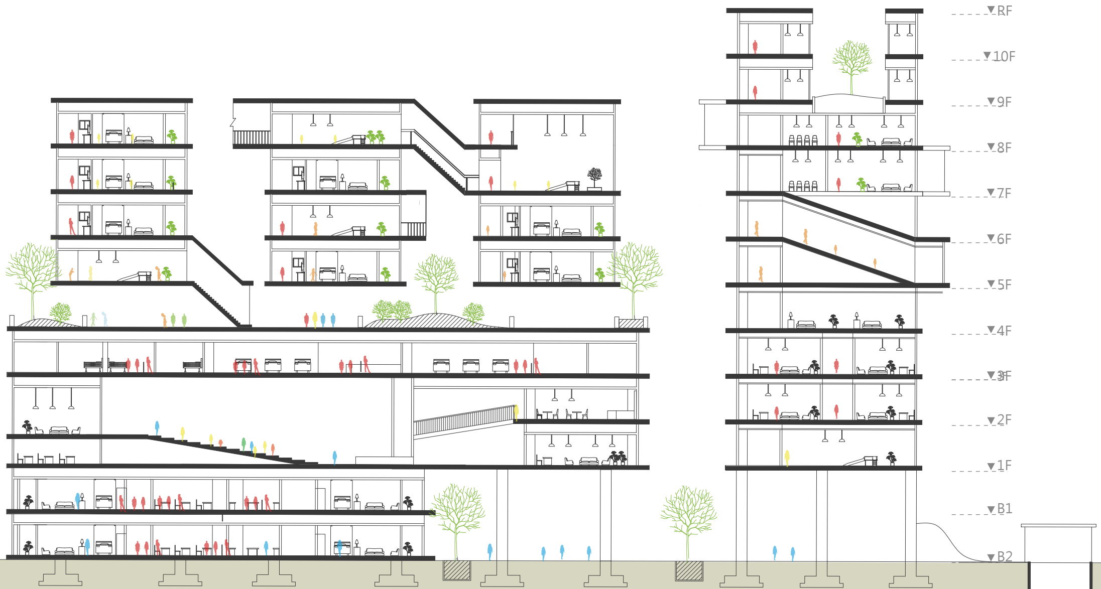
SECTION OF WARD BUILDING
