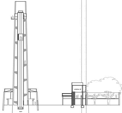
Housing-C South-elevation
