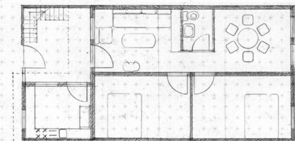
1F plan
