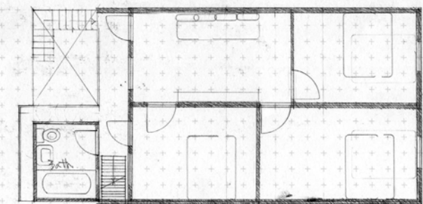
2F plan
