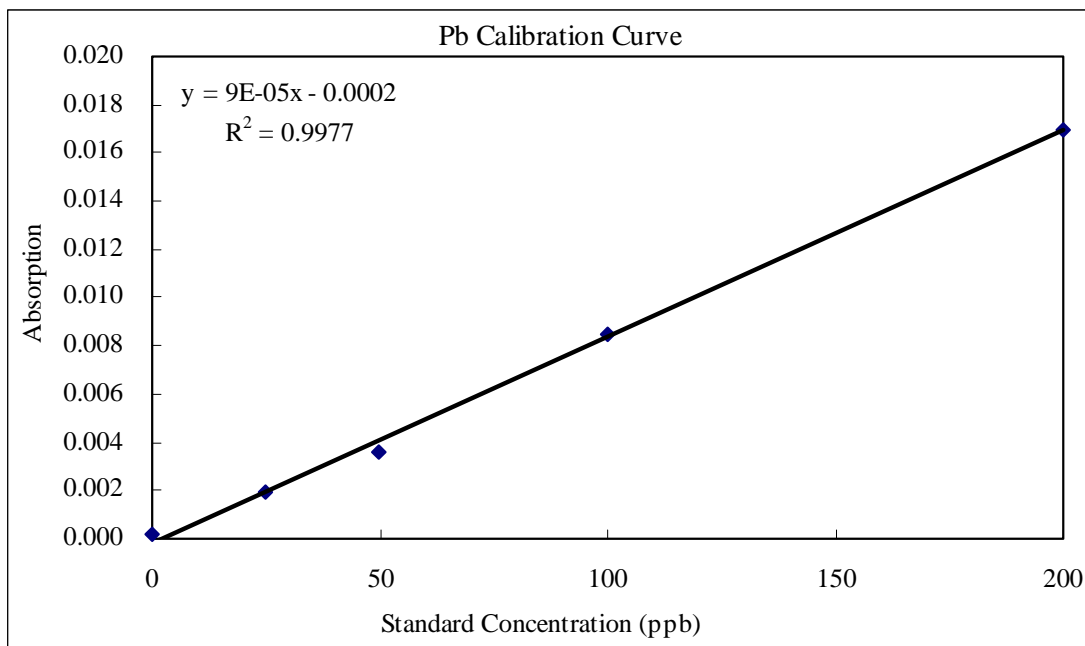
Figure A-5 The calibration curve of Pb.
