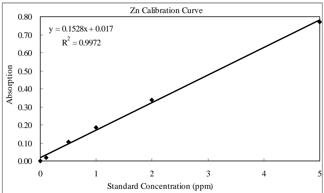
Figure A-4 The calibration curve of Zn.
