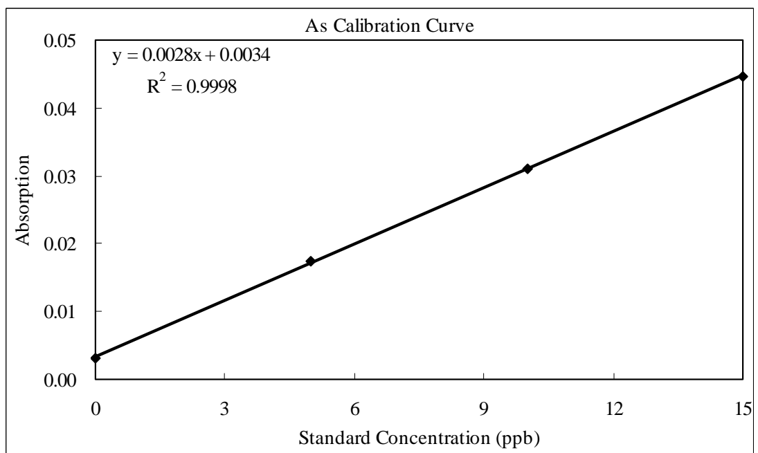
Figure A-10 The calibration curve of As.
