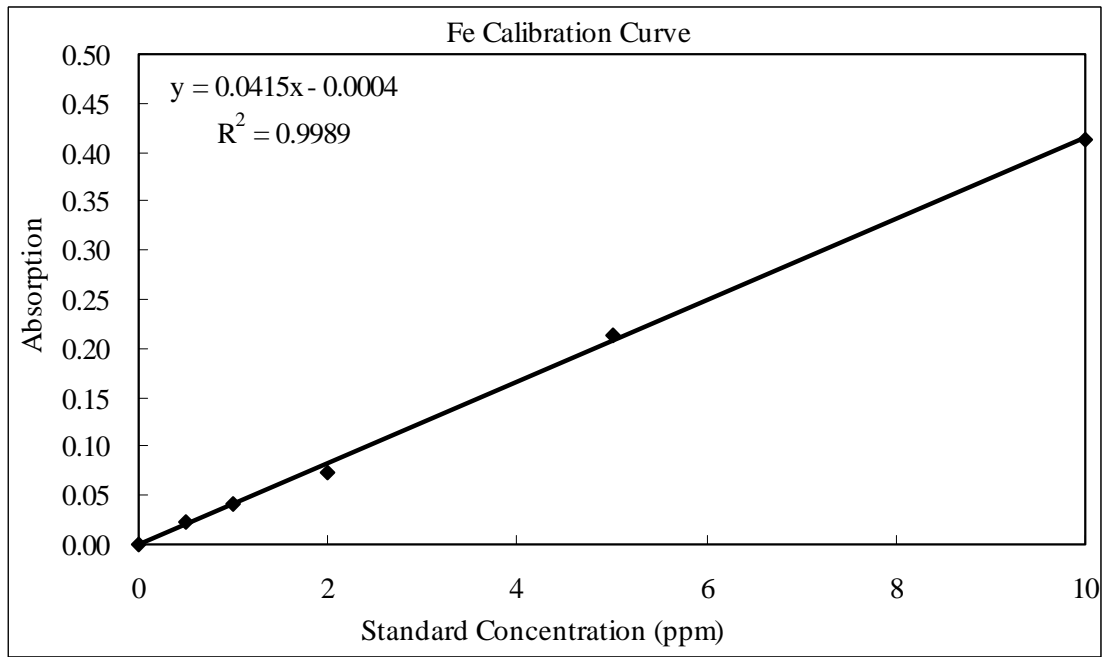
Figure A-1 The calibration curve of Fe.
