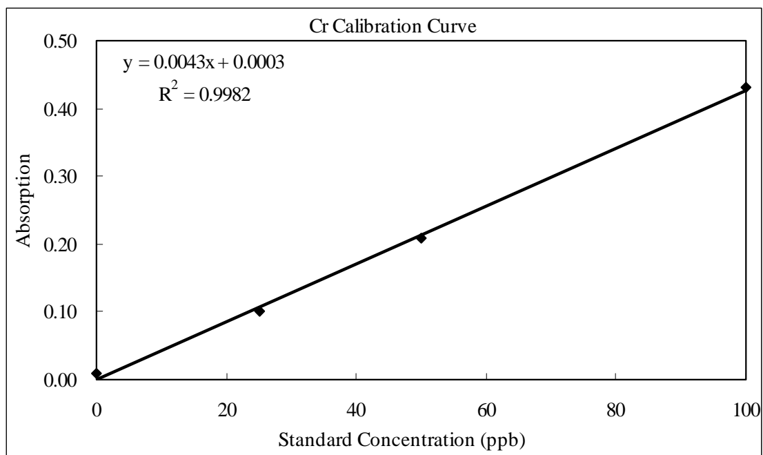
Figure A-6 The calibration curve of Cr.
