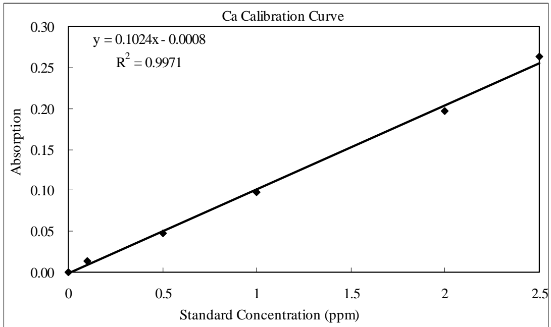
Figure A-3 The calibration curve of Ca.
