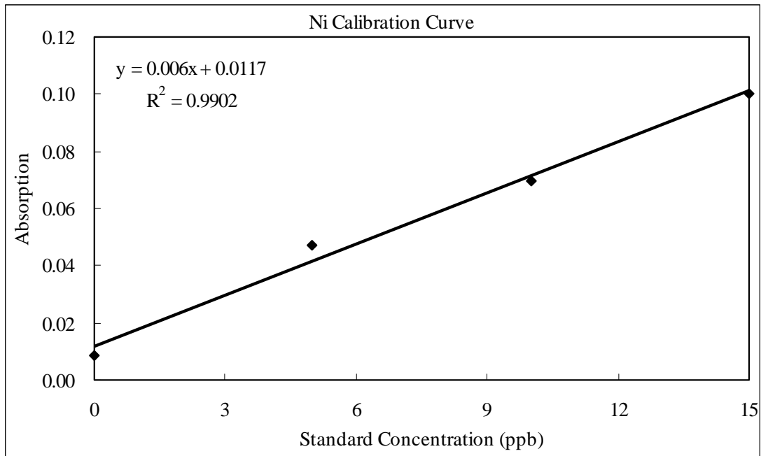
Figure A-11 The calibration curve of Ni.
