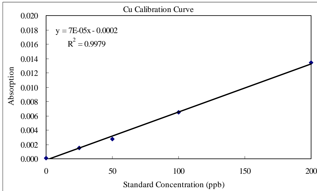
Figure A-8 The calibration curve of Cu.
