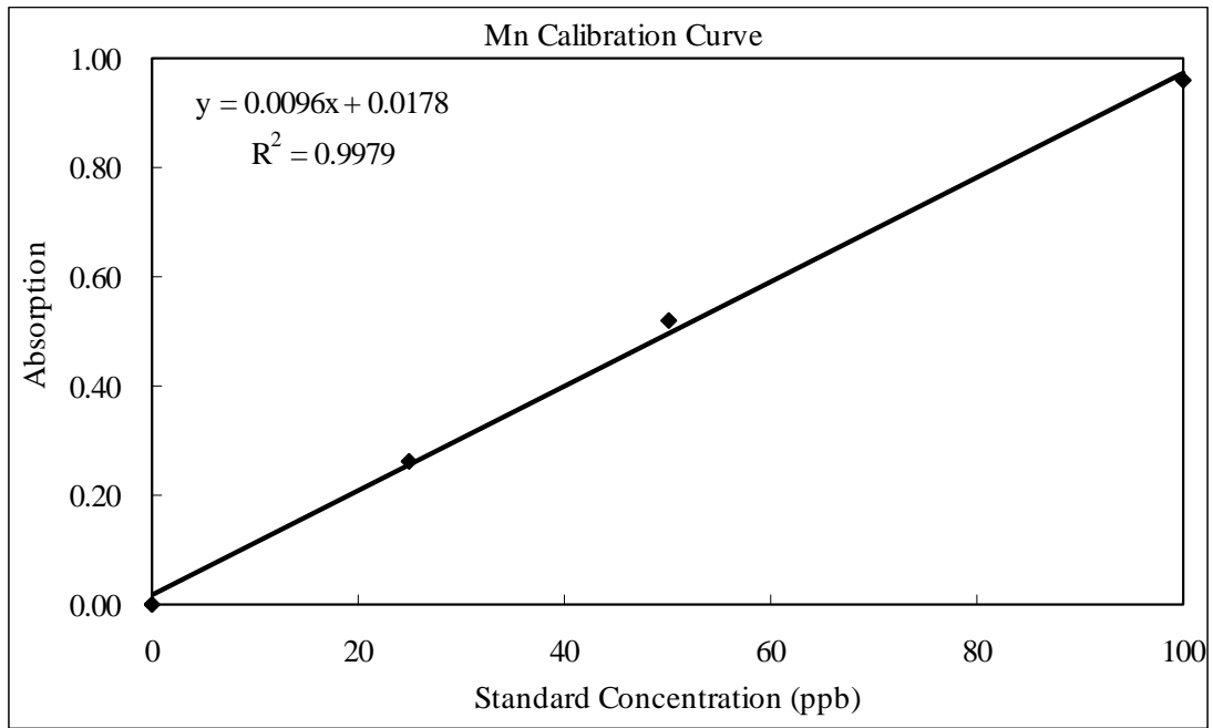
Figure A-9 The calibration curve of Mn.
