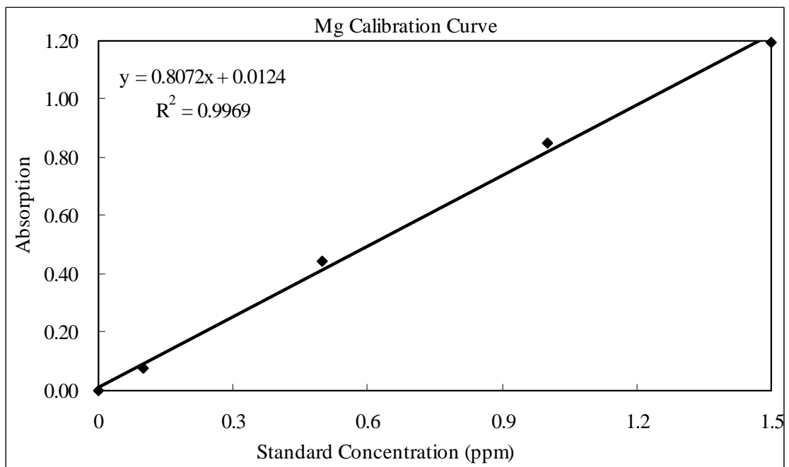
Figure A-2 The calibration curve of Mg.
