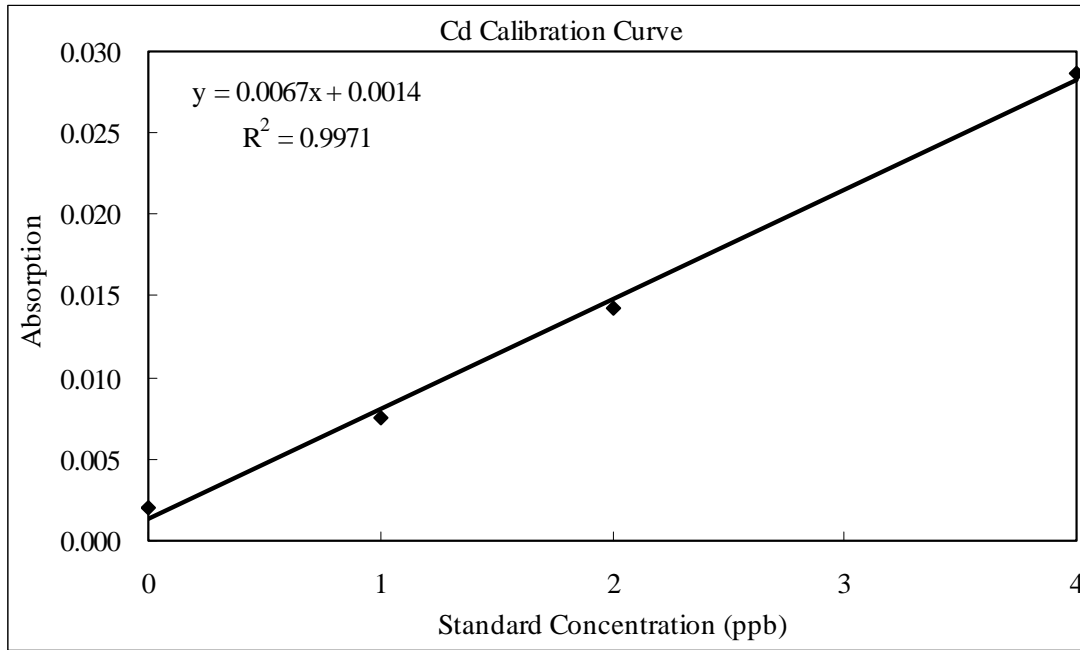
Figure A-7 The calibration curve of Cd.
