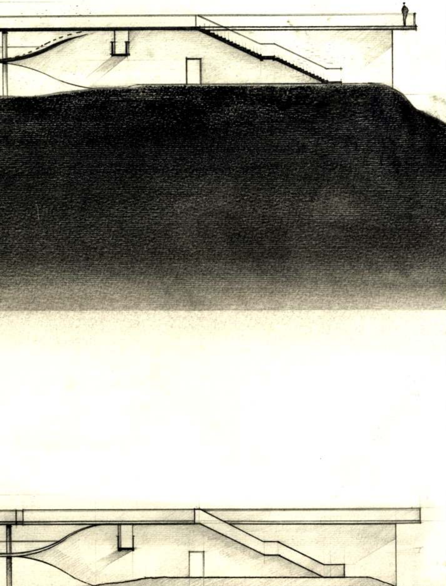
Changing Room FF' Section South Elevation
